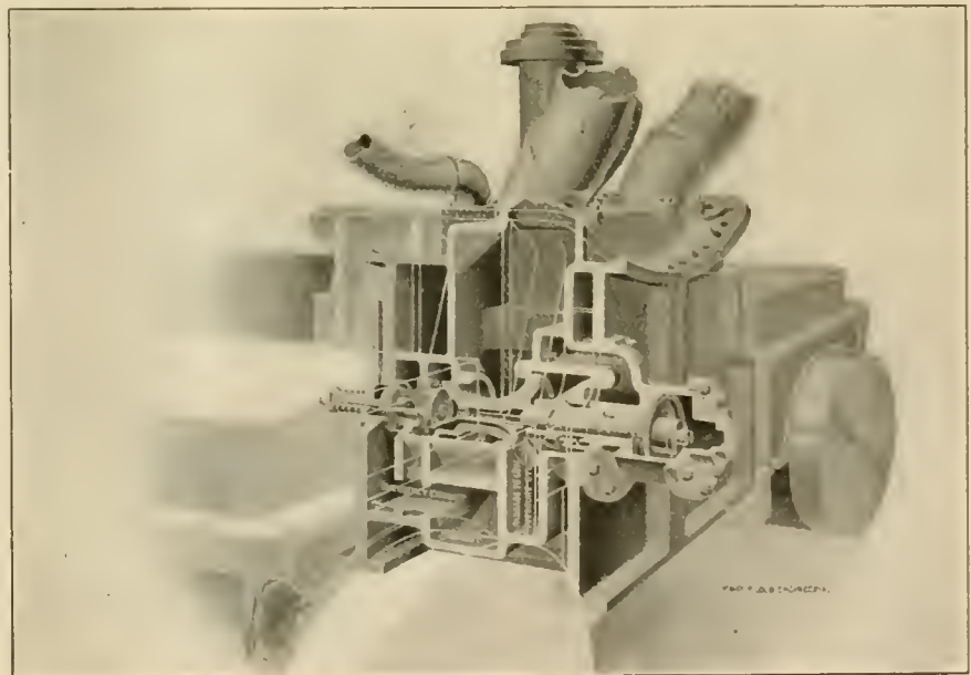
RICHMOND COMPOUND—INTERCEPTING VALVE IN SIMPLE POSITION
